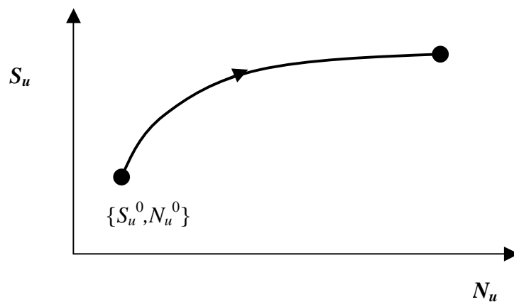
Fig. 1.6. Trajectory of the city evolution.
