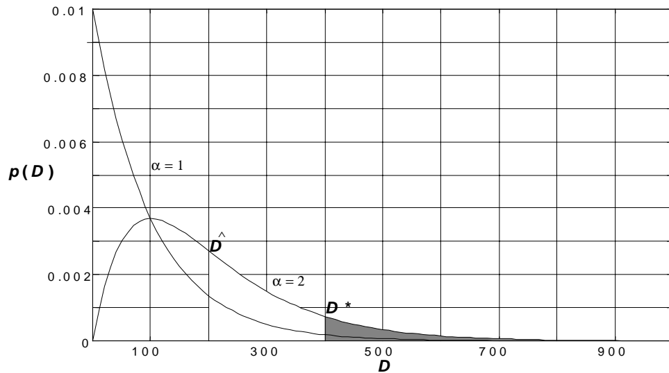
Fig. 1.7. \Gamma - distribution as the distribution with density p(D) .
