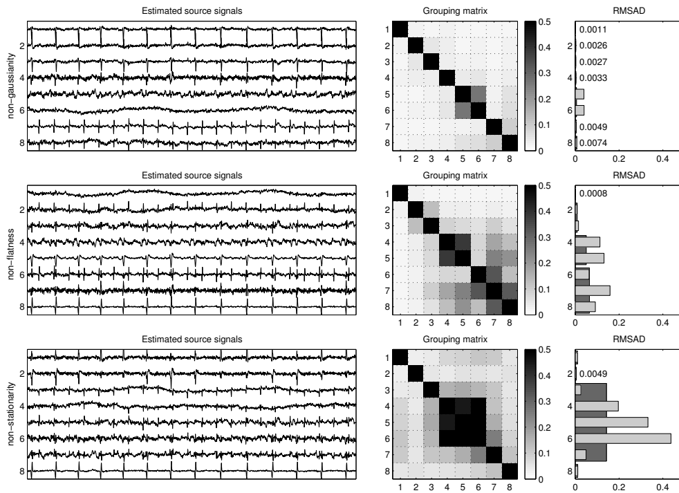
Figure 3.6: Shown are the results for the fetal ECG. As explained in the text, the extracted components from the ICA algorithm based on non-Gaussianity are the most reliable. For the first row we used JADE, for the second row we used TDSEP with time-lags 0, \dots, 20 , for the third we used SEPAGAUS being restricted to one positive frequency channel.
