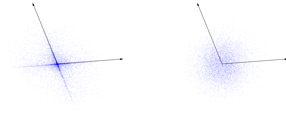
Figure 3.1: Can you trust your independent components? Left panel: the chosen directions reflect the underlying statistical structure of the data; right panel: the data is rotation-invariant, so any other directions could have been chosen.
