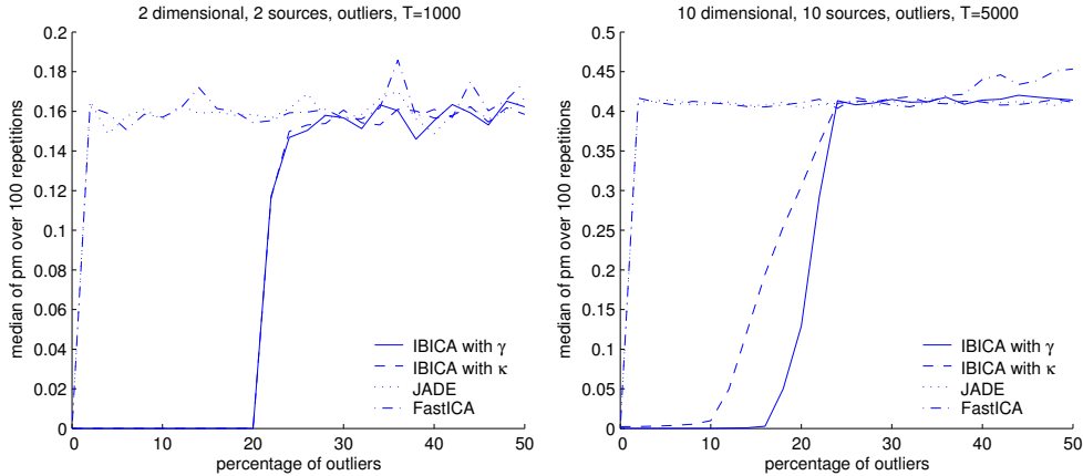
Figure 4.5: IBICA is very robust with respect to outliers: replacing a significant amount of the data with outliers does not change the result of IBICA (left panel: two dimensions; right panel: 10 dimensions).
