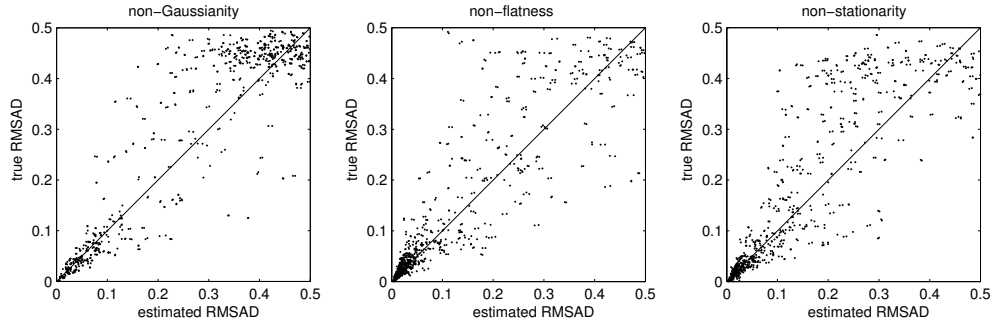
Figure 3.4: The estimated RMSAD correlates in all three cases with the true RMSAD. Note, that these scatterplots depend on the choice of the noise parameter \chi . All experiments have been carried out with \chi = \pi/8 .
