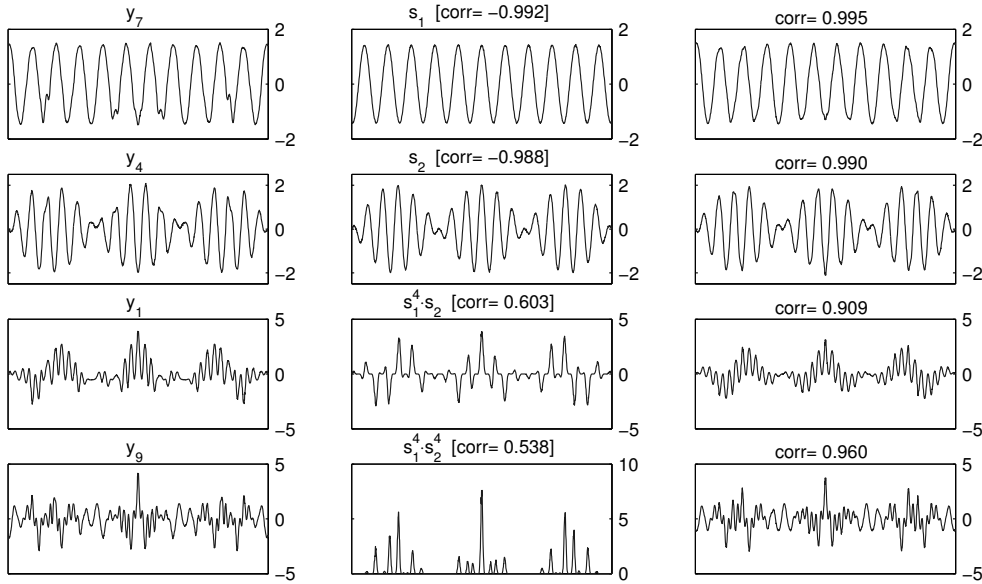
Figure 5.6: The extracted signals in the left panels (only four shown) are tried to be matched with single quasi sources in the middle panels and combinations of subgroups of quasi sources (right panels).
