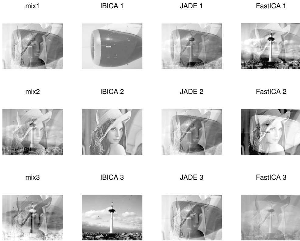
Figure 4.12: IBICA is able to separate mixed images (first column) that have been contaminated with outliers (black pixels in the images of the first columns) after sparsifying the data with a wavelet transformation as the images in the middle column show. JADE and FastICA fail (third and fourth column).
