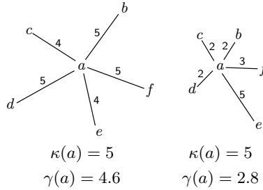
Figure 4.2: Because \gamma takes into account all k nearest neighbors and not only the k -th like \kappa does, \gamma can distinguish better between sparse and dense regions than \kappa for k = 5 .
