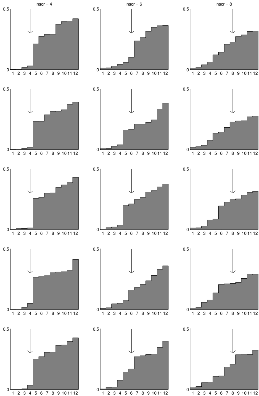
Figure 4.7: If the number of sources is not known, large gaps in the stairs plots of \zeta_1, \dots, \zeta_{12} can help. Shown are the stairs plot for the examples in Figure 4.6. Up to four sources the true number of sources can be identified, see also Figure 4.8.
