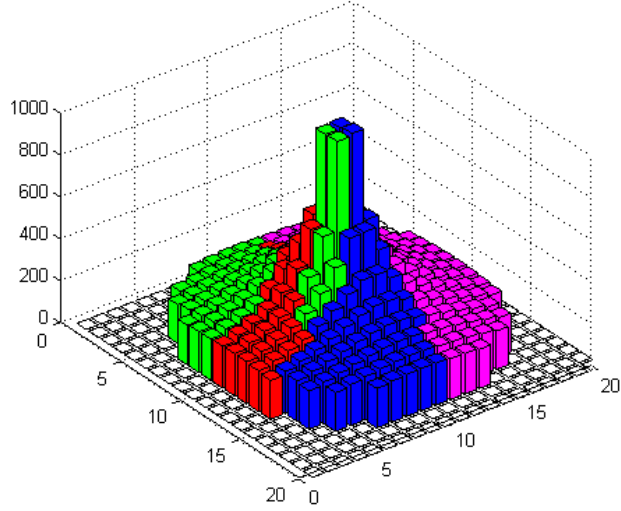
Figure 3: Density of four household groups with symmetric socioeconomic variables in a monocentric city
